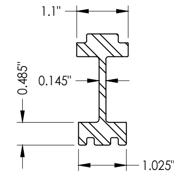
11 MULLION REINFORCEMENT
