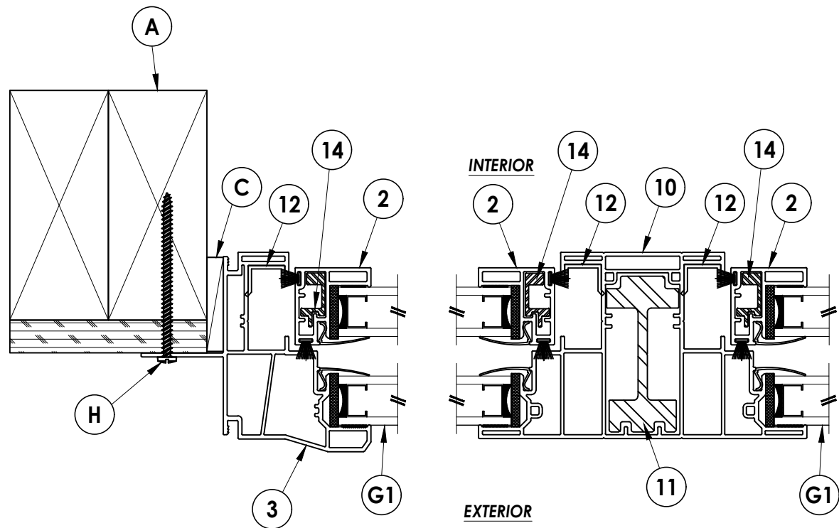
1 HORIZONTAL CROSS SECTION 3 Stud Construction
