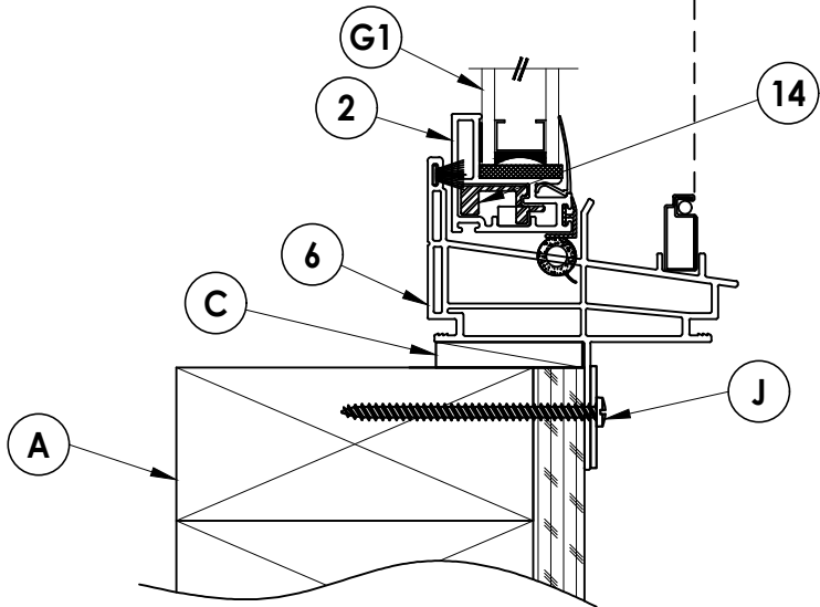
2 VERTICAL CROSS SECTION 3 Stud Construction
